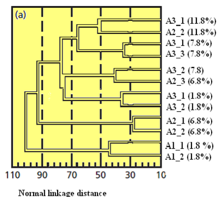
Figure 1a. Dendrogram of the cluster analysis on the profiles of respiratory quinones, And cellular fatty acids.
