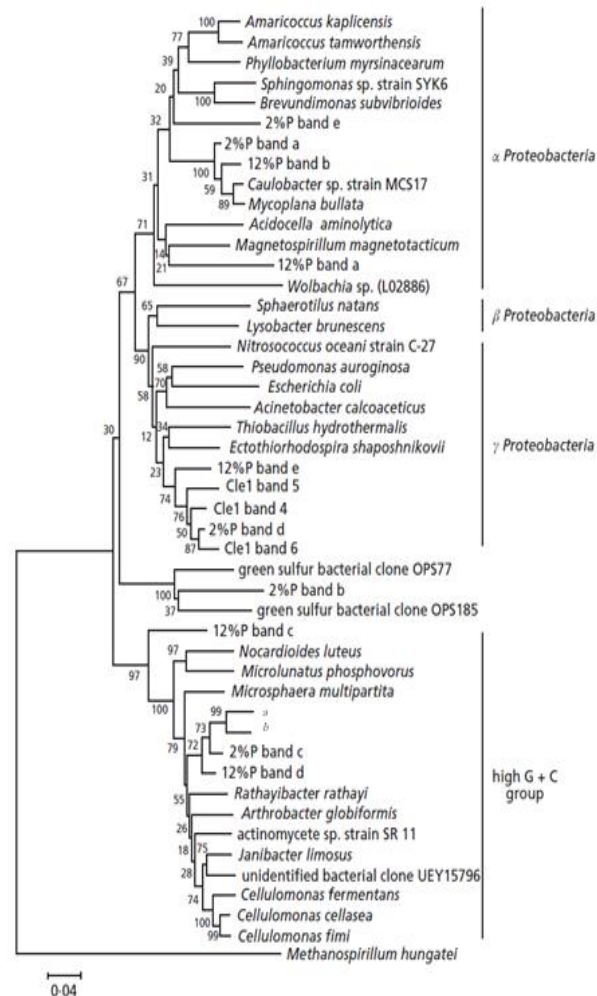
Figure 3. phylogenetic distribution of numerically dominant populations in sludge samples containing either 2% or 12.3% P, based on the partial sequence of 16S rDNA genes resolved using DGGE.
