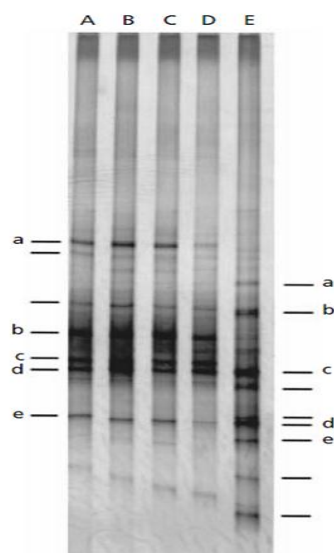
Figure 2. Polymerase chain reaction-Denaturing gradient gel electrophoresis analysis of activated sludge sample.
