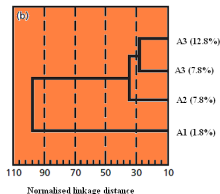
Figure 1b. Dendrogram of the cluster analysis on the profiles of respiratory quinones, For samples containing different sludge P contains.
