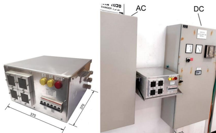
Figure12. Automatic HEMP protected charger for auxiliary DC power supply systems of critical infrastructures
