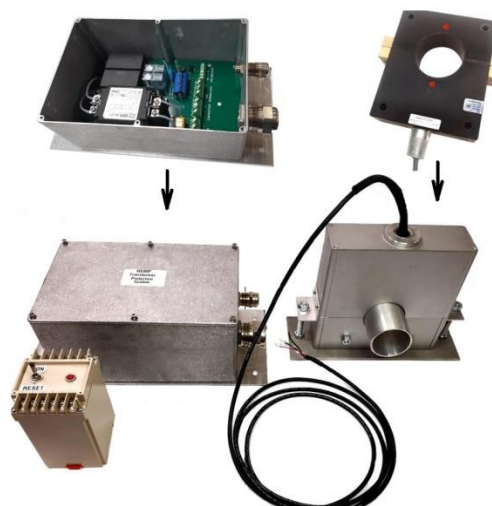
Figure10. Simple system for protection of high-power transformer against E3 component of HEMP
