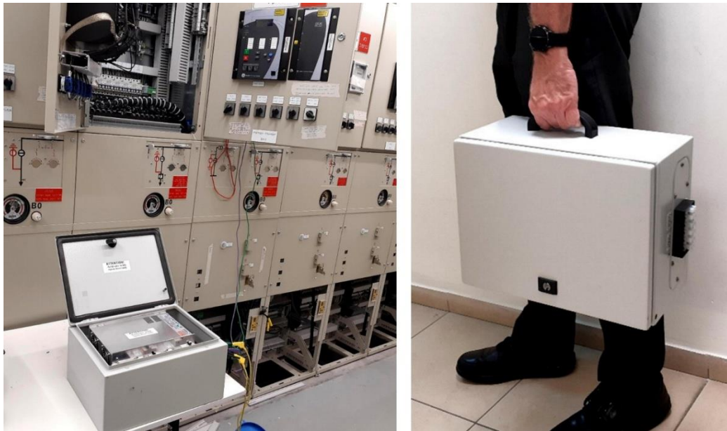
Figure14. HEMP protected backup power supply for electronic equipment testing after HEMP impact
