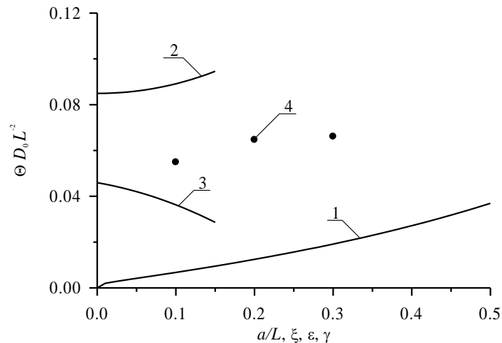
Fig5b. Dimensionless optimal annealing time of implanted dopant as a function of several parameters. Curve 1 describes the dependence of the annealing time on the relation a/L and \xi = \gamma = 0 for equal to each other values of dopant diffusion coefficient in all parts of heterostructure. Curve 2 describes the dependence of the annealing time on value of parameter \epsilon for a/L=1/2 and \xi = \gamma = 0 . Curve 3 describes the dependence of the annealing time on value of parameter \xi for a/L=1/2 and \epsilon = \gamma = 0 . Curve 4 describes the dependence of the annealing time on value of parameter \gamma for a/L=1/2 and \epsilon = \xi = 0
