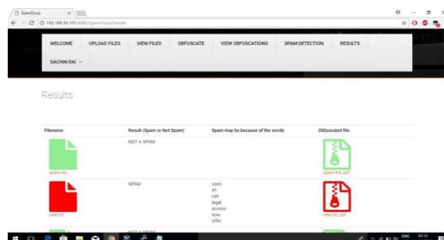
Fig9. Results Page
