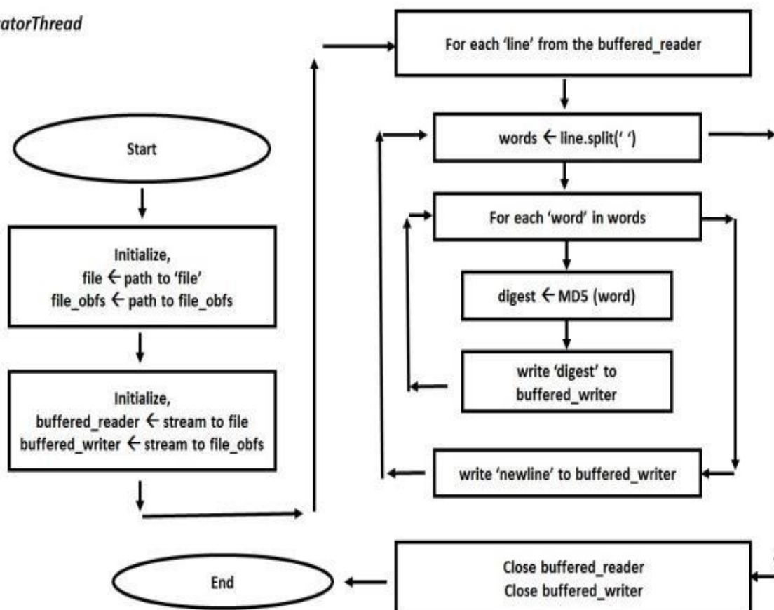
Fig4. Obfuscator thread
