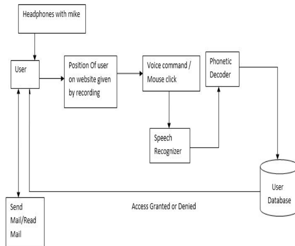
Fig2. Level 2 DFD
