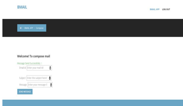
Fig5. Compose Page
