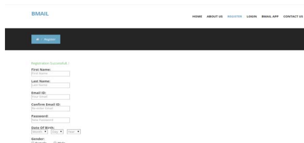
Fig3. Registration Page
