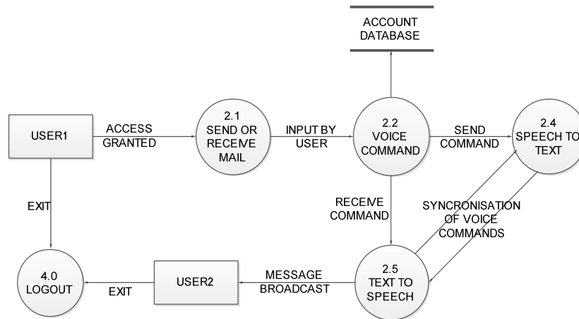
Fig1. System architecture
