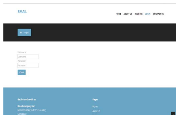
Fig4. Login Page
