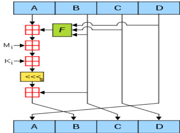
Fig7. Structure of Message Digest Algorithm
