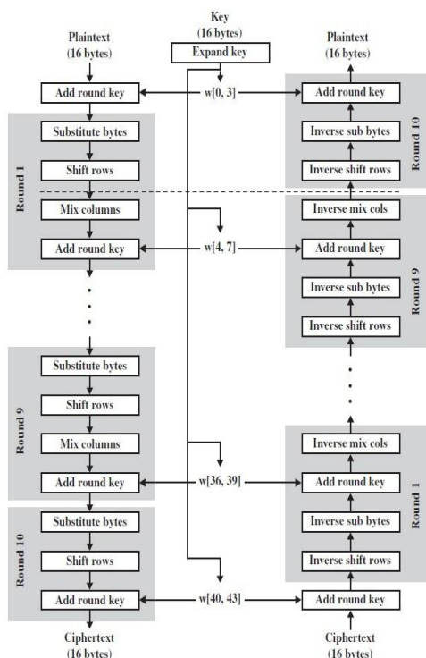
Fig5. Structure of Advance Encryption Standard Algorithm
