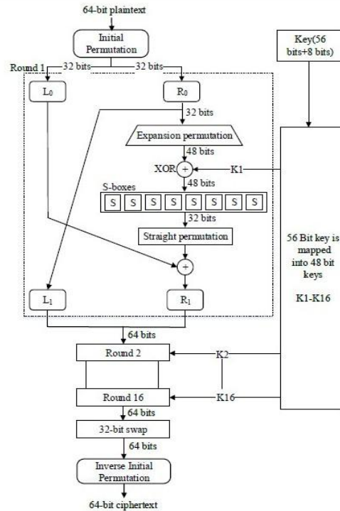
Fig3. Structure of DES
