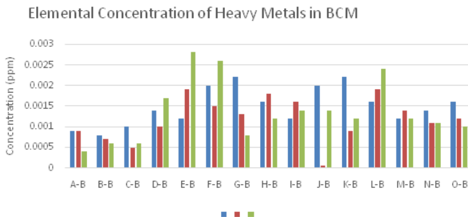
Fig7. Comparison of concentrations (ppm) of heavy metals of all BCM samples
