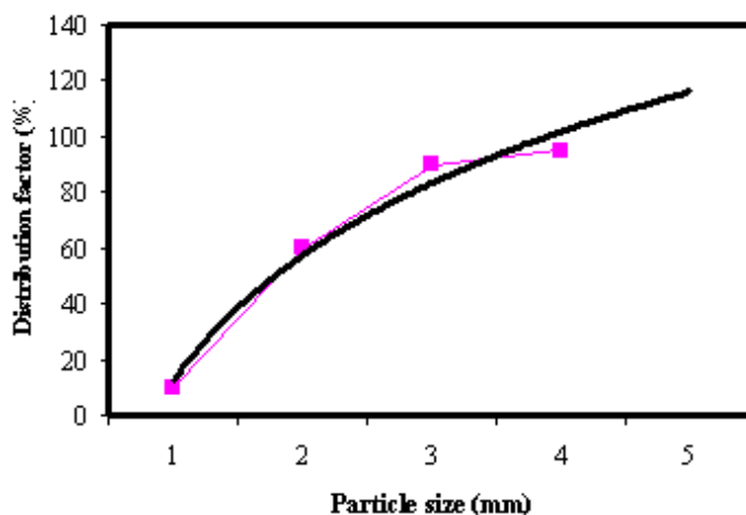
Figure9. The variation of distribution factor against particle size for coal undersizes in a classifier. The sizes correspond to mid-point for ranges 5. Green heat
