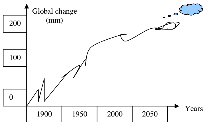
Figure4. Change in global sea level [11].
