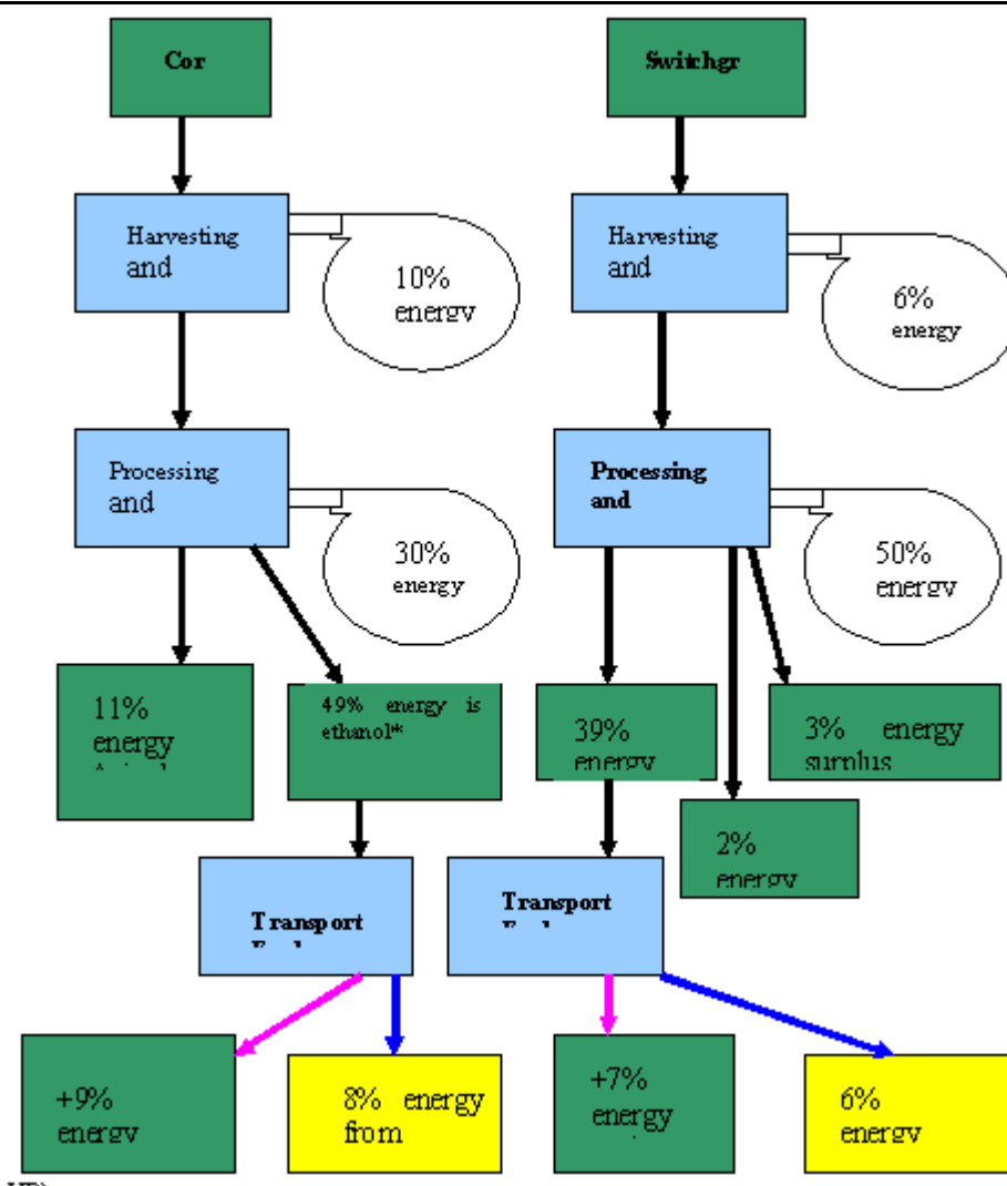
Figure 8. The lifecycle energy balance of corn and Switchgrass reveal a paradox: corn, as an ethanol feedstock requires less energy for production, i.e., more of the original energy in starch is retained in the ethanol fuel. Nevertheless, the Switchgrass process yields higher GHG emissions. This is because most of the process energy for Switchgrass process is generated from GHG emission neutral biomass residue.
