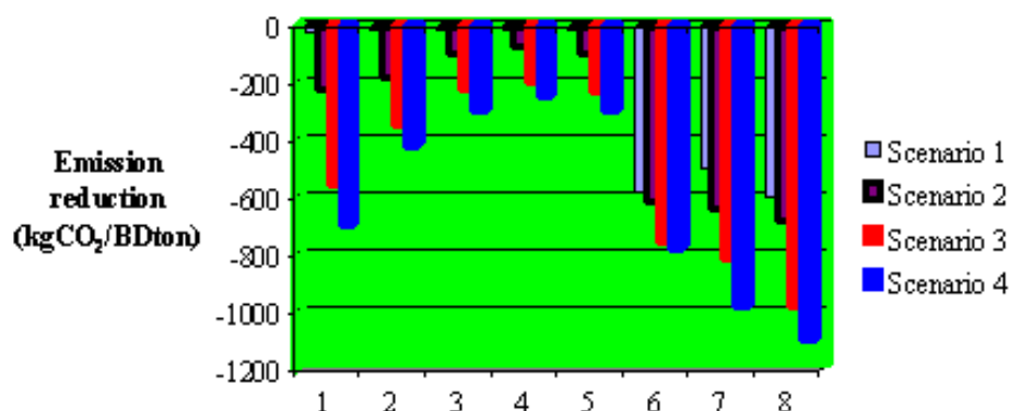
Figure 7. Comparison of thermal biomass usage options, CHP displacing natural gas as a heat source
