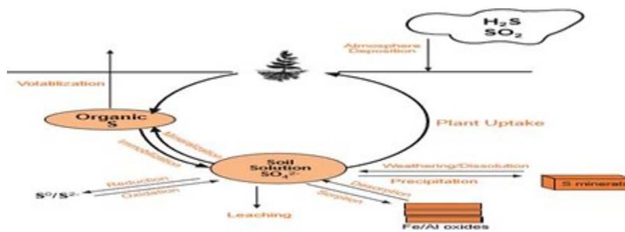
Figure1. Sulfur Cycle
