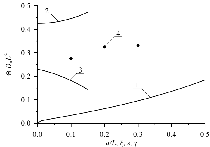
Fig5a. Dimensionless optimal annealing time of infused dopant as a function of several parameters. Curve 1 describes the dependence of the annealing time on the relation a/L and \xi = \gamma = 0 for equal to each other values of dopant diffusion coefficient in all parts of heterostructure. Curve 2 describes the dependence of the annealing time on value of parameter \varepsilon for a/L=1/2 and \xi = \gamma = 0 . Curve 3 describes the dependence of the annealing time on value of parameter \xi for a/L=1/2 and \varepsilon = \gamma = 0 . Curve 4 describes the dependence of the annealing time on value of parameter \gamma for a/L=1/2 and \varepsilon = \xi = 0
