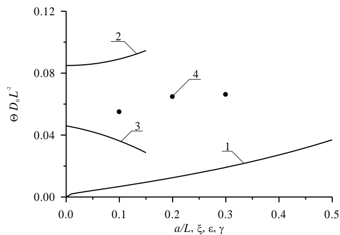
Fig5b. Dimensionless optimal annealing time of implanted dopant as a function of several parameters. Curve 1 describes the dependence of the annealing time on the relation a/L and \xi = \gamma = 0 for equal to each other values of dopant diffusion coefficient in all parts of heterostructure. Curve 2 describes the dependence of the annealing time on value of parameter \varepsilon for a/L=1/2 and \xi = \gamma = 0 . Curve 3 describes the dependence of the annealing time on value of parameter \xi for a/L=1/2 and \varepsilon = \gamma = 0 . Curve 4 describes the dependence of the annealing time on value of parameter \gamma for a/L=1/2 and \varepsilon = \xi = 0
