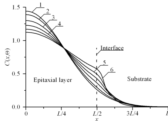
Fig2a. Dependences of concentration of dopant, infused in heterostructure from Figs. 1, on coordinate in direction, which is perpendicular to interface between epitaxial layer substrate. Difference between values of dopant diffusion coefficient in layers of heterostructure increases with increasing of number of curves. Value of dopant diffusion coefficient in the epitaxial layer is larger, than value of dopant diffusion coefficient in the substrate
