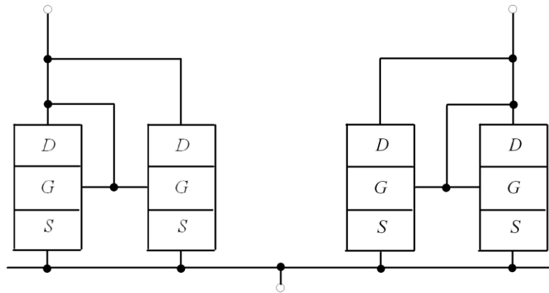
Fig1. The considered current comparator [4]
