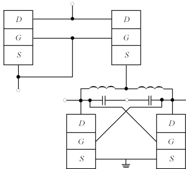
Fig1. The considered injection locked oscillator [4]
