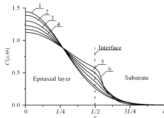
Fig2. Distributions of concentration of infused dopant in heterostructure from Fig. 1 in direction, which is perpendicular to interface between epitaxial layer substrate. Increasing of number of curve corresponds to increasing of difference between values of dopant diffusion coefficient in layers of heterostructure under condition, when value of dopant diffusion coefficient in epitaxial layer is larger, than value of dopant diffusion coefficient in substrate
