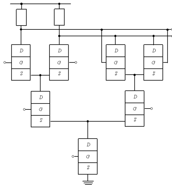
Fig1a. Structure of the considered logic gate [19]
