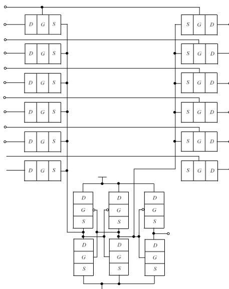
Fig1. The considered bit-cell circuit [4]
