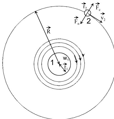
Fig1. Two-dimensional model of gravitational interaction of two bodies. The forces are shown acting on body 2: F_c – the centrifugal force, F_n – the force of attraction of body 2 from body 1; v_2 – linear velocity of body 2 at the orbit, R – the radius of the orbit, r_1 – the radius of body 1, r_2 – the radius of body 2, w_1 – angular velocity of ether rotation at the surface of body 1, and m_2 are the mass of body 2.
