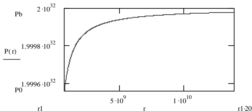
Fig2. Radial distribution of pressure in the ether torsion
