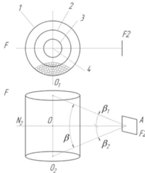
Figure4. Radiation of cylindrical gas volume on the calculated area F_2
