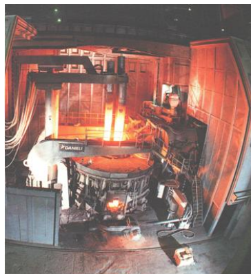
Figure1. Arc Steel Furnace
