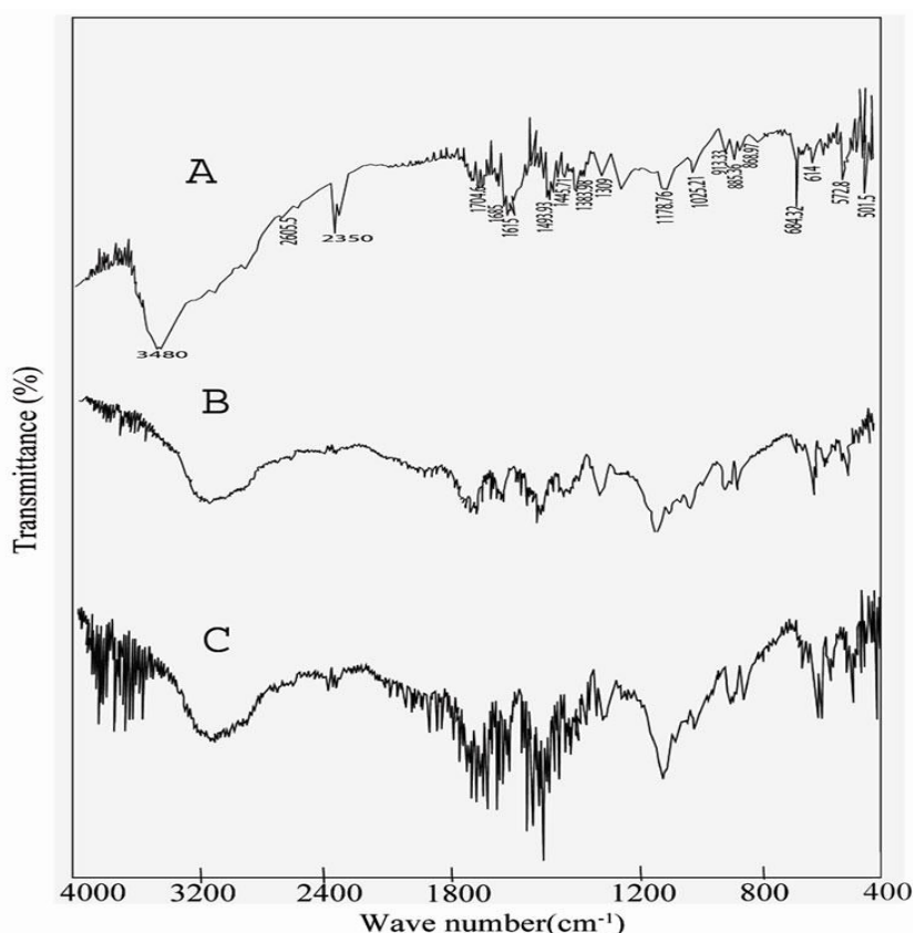
Fig4. FTIR Spectra (A) pure TGS (B) 0.5 mole% methyl orange doped TGS and (C) 0.5 mole% methyl red doped TGS Crystal.
