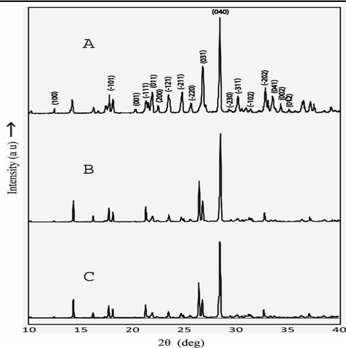
Fig2. X-ray powder diffraction pattern for (A) pure TGS (B) 0.5 mole% methyl orange doped TGS and (C) 0.5 mole% methyl red doped TGS crystal.
