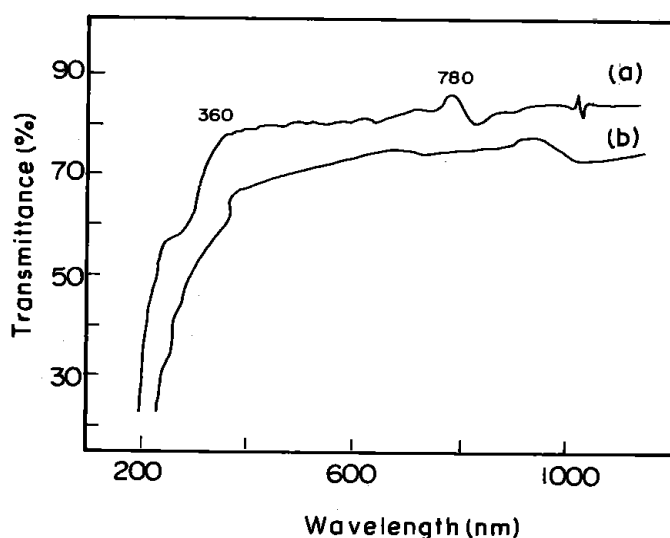
Fig3. UV-Visible transmittance spectra for (a) Pure TGS, (b) TGS + 0.5 mole% of methyl orange doped TGS crystals.
